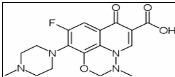
Figure 1: Marbofloxacin formula
