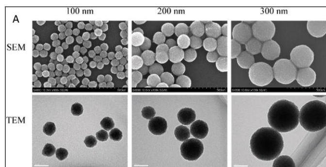
Figure II. Morphological characterization and structure diagram of TiO 2 PEG nanoparticles of different sizes. TiO 2 -PEG nanoparticles 100, 200, and 300 nm in size were characterized by SEM (upper panels) and TEM (lower panels). Both SEM and TEM images showed that the nanoparticles were spherical and uniform. The characterization of TiO 2 -PEG NPs confirmed the enhancement effect of PEG-glycation on the dispersity and uniformity of TiO 2 NPs [23].
